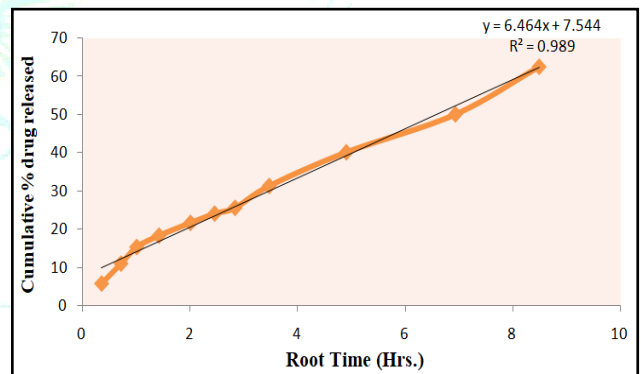
Figure 11 Graph of Higuchi release Kinetics of transfersome gel TF2
