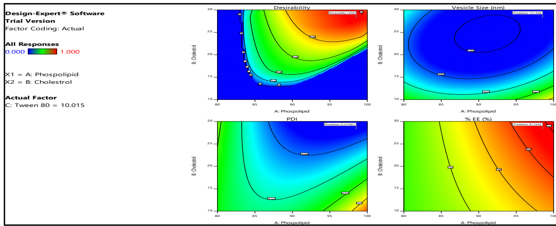
Figure 7 Contour plots for all parameters
