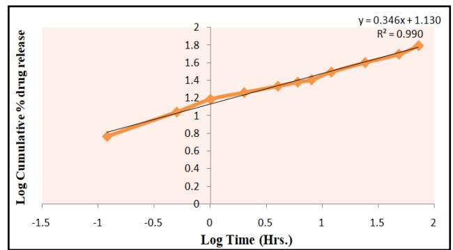
Figure 12 Graph of Korsmeyer-Peppas release Kinetics of transfersome gel TF2
