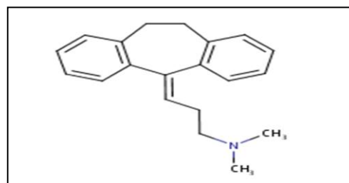
Figure 2: Amitriptyline Hydrochloride
